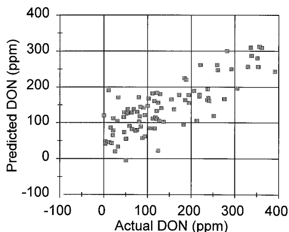
Fig. 3. Single wheat kernel deoxynivalenol (DON) levels predicted using near-infrared spectroscopy (NIRS).
