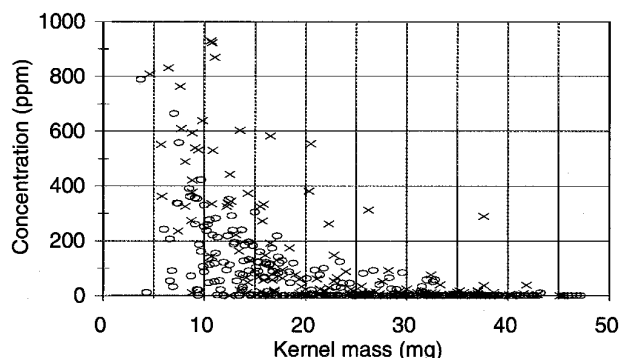
Fig. 5. Relationship between single kernel weight and levels of deoxynivalenol (DON) (○) and ergosterol (×).
